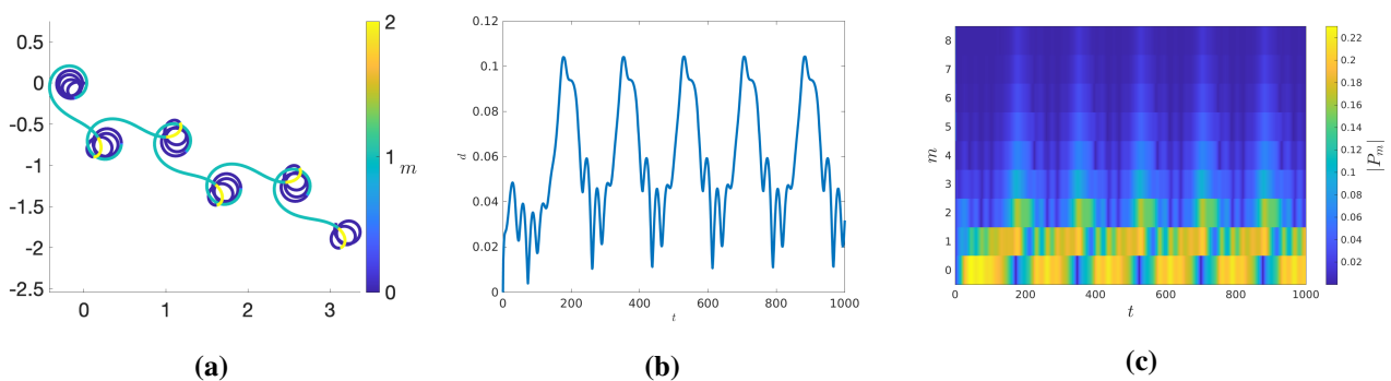
Figure 17. Dynamics of an active droplet with coupling between dominant m = 0 and m = 1 modes with (\alpha, \beta, \zeta) = (-2.6, 0.2, 0.1) and (d_T, d_R, Ca) = (0.05, 0.05, 1) . (a) Trajectory of the droplet center. (b) Drop deformation number d as a function of time. (c) A contour plot of |P_m| (absolute Fourier amplitude of the vorticity along \Gamma_t ).
