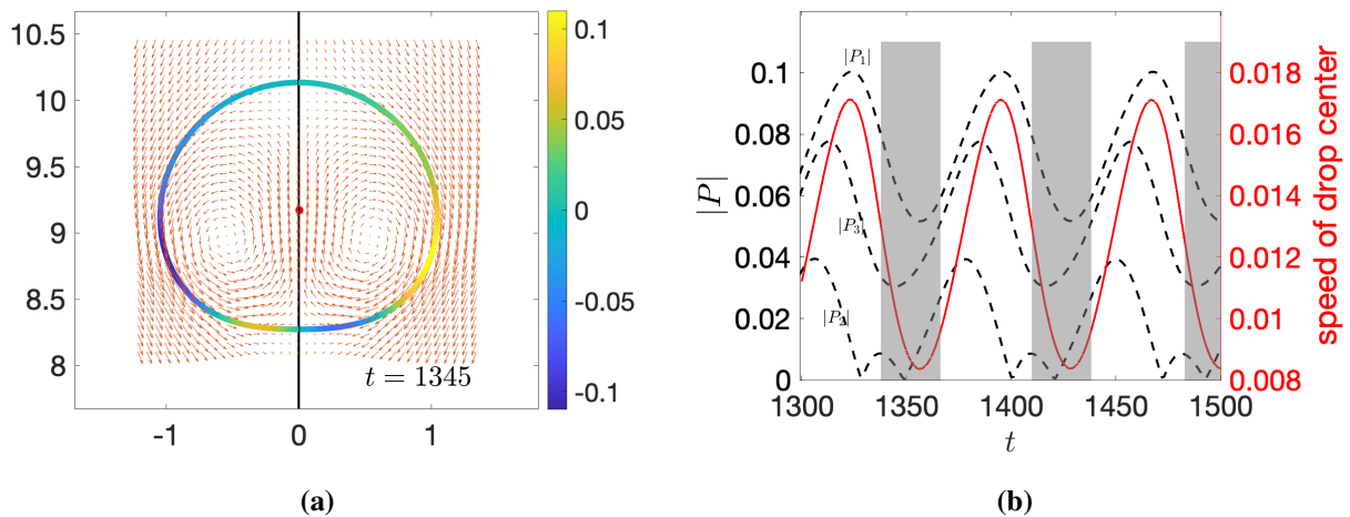
Figure 23. Pulsating dynamics of a contractile drop ( \alpha > 0 ). (a) Flow field in the comoving frame of the drop center at t = 1345 , with the drop boundary color-coded by the vorticity on \Gamma_r . (b) Correlation between Fourier amplitudes of vorticity on the surface (dashed curves for |P_1| , |P_2| , |P_3| as labeled), the center-of-mass speed (solid curve, right axis) and defect activity (grey regions).
