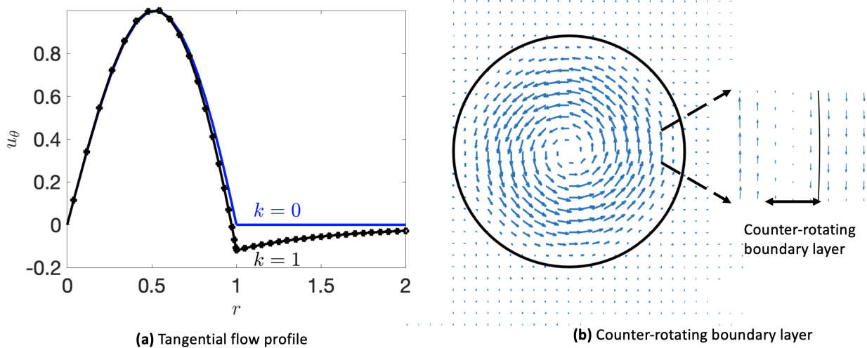
Figure 25. Flow field of an active drop with bottom friction. \alpha = -2.212 , \beta = 0.6 , \zeta = 1.5 , d_T = 0.05 , and d_R = 0.05 . (a) u_\theta between Stokes flow ( k = 0 , blue curve) and Brinkman flow ( k = 1 , black curve with squares) constructed from the linear solution. (b) Illustration of the counter-rotating boundary layer.
