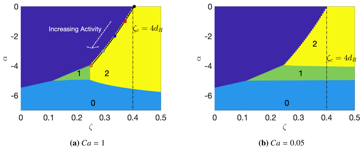
Figure 4. Regions where different azimuthal modes dominate in the (\alpha, \zeta) plane at two different capillary numbers. The dominant mode number is labeled when any mode is unstable. No azimuthal mode is unstable in the purple region. For both panels, d_T = 0.1 , d_R = 0.1 , and \beta = 0.2 . Capillary numbers are indicated in the subcaptions.
