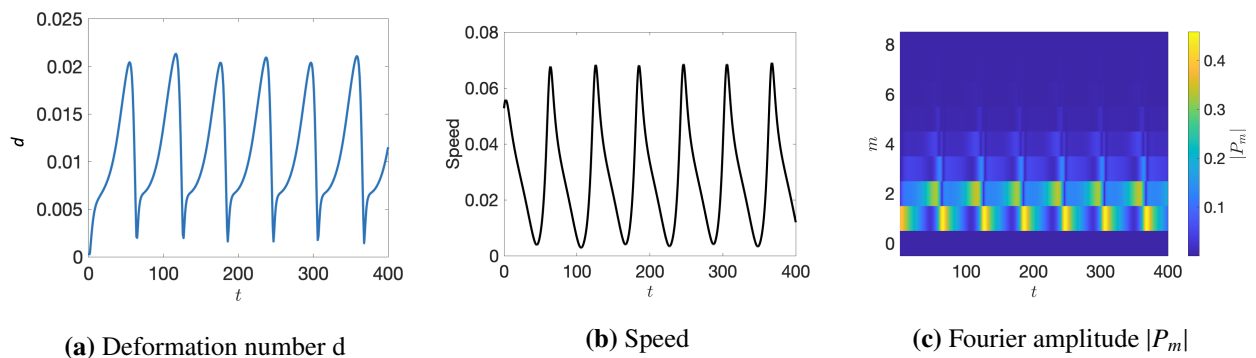
Figure 14. Nonlinear dynamics for a drop with the m = 1 and m = 2 modes unstable. Here \alpha = -4 , \beta = 1 , \zeta = 0.56 , d_T = 0.1 , d_R = 0.16 and Ca = 0.1 . Panel (a) shows the drop deformation number d as a function of time. Panel (b) shows the speed of the drop center of mass as a function of time. Panel (c) shows a contour plot of |P_m| (absolute Fourier amplitude of the vorticity along the drop interface).
