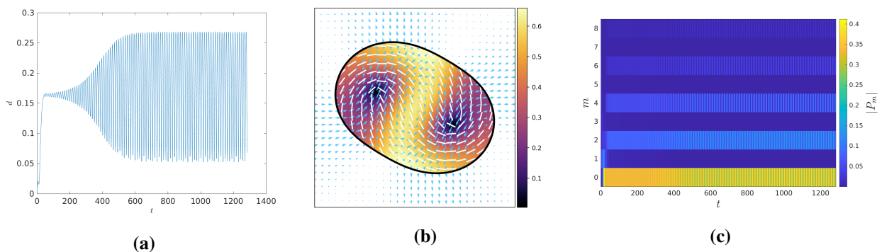
Figure 15. Nonlinear dynamics for a wobbling washing machine. Here \alpha = -2.4 , \beta = 0.2 , \zeta = 0.123 , d_T = 0.05 , d_R = 0.05 , Ca = 1 and initial drop radius = 1.75. Panel (a): oscillation of drop deformation that corresponds to the wobbling. Panel (b): the fluid velocity field and the nematic order parameter. Panel (c): a contour plot of |P_m| (the absolute Fourier amplitude of the vorticity along the interface).
