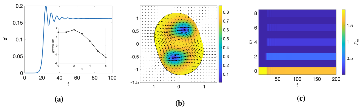
Figure 16. Nonlinear dynamics for a m = 2 dominant drop seeded with a rotational ( m = 0 ) mode. Here \alpha = -5.5 , \beta = 1 , \zeta = 1.5 , d_T = 0.11 , d_R = 0.08 and Ca = 1 . Panel (a) shows the drop deformation number d as a function of time, and the insert shows the growth rate. Panel (b) shows the fluid velocity field and the scalar order parameter. Panel (c) is a contour plot of |P_m| (absolute Fourier amplitude of the vorticity on the drop interface).
