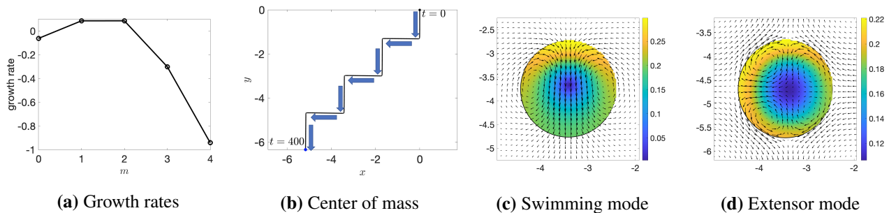
Figure 13. Nonlinear dynamics for a drop with the m = 1 and m = 2 modes unstable. Here \alpha = -4 , \beta = 1 , \zeta = 0.56 , d_T = 0.1 , d_R = 0.16 and Ca = 0.1 . Panel (a) shows the linear growth rate as a function of the azimuthal wavenumber m . Panel (b) shows the trajectory of the drop center from t = 0 to t = 400 . Panels (c) and (d) show the scalar order parameter (contour plot) and the flow field at different points in time. Panel (c) is at t = 250 , during the “swim” phase, and the drop dynamics are dominated by the m = 1 mode; panel (d) is at t = 290 , in an asymmetric extensor mode, with the drop dynamics dominated by m = 2 mode.
