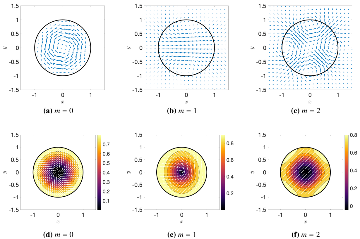
Figure 2. Reconstructed eigenfunctions associated with the m = 0 (panels a, d), m = 1 (panels b, e), and m = 2 (panels c, f) modes for \alpha = -4 , \beta = 0.2 , \zeta = 0.1 , d_R = 0.1 , d_T = 0.1 , and Ca = 1 . Panels (a–c) show the flow fields, panels (d–f) show the nematic field. White lines give the orientation of the director field; color scale shows the scalar nematic order parameter.
