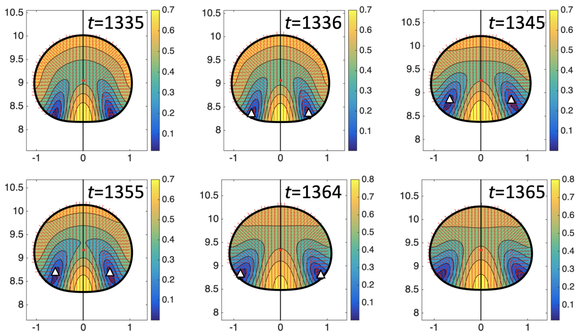
Figure 24. Birth and death of a pair defects (white triangles) for a contractile active drop with \alpha = 1 , \beta = 0.1 , \zeta = 0.2 , d_T = 0.01 , d_R = 0.02 and Ca = 1 . Contour plots of the scalar order parameter are over plotted with arrows of the dominant eigenvectors of \mathbf{D} at different times as labeled. Red dots denote the drop center, and triangles denote the defect locations where the scalar order parameter is nearly zero.
