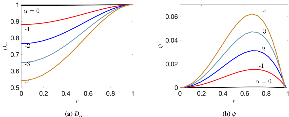
Figure 5. Radial dependence of the eigenfunction for the extensor mode, with \zeta = 0.1 , d_T = 0.1 , d_R = 0.1 , Ca = 1 , and \beta = 0.2 . D_{rr} is shown in panel (a) and the streamfunction \psi is shown in panel (b).
