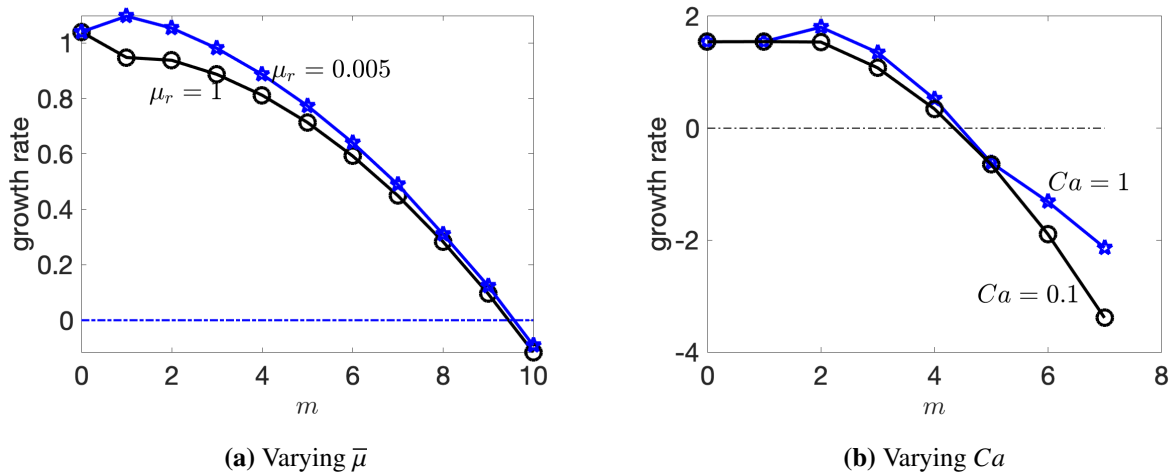
Figure 3. Effect of viscosity contrast \bar{\mu} and surface tension Ca on the linear growth rate. Panel (a): Growth rate for \bar{\mu}_r = 1 (circles) and \bar{\mu} = 0.005 (stars) with \alpha = -1 , \beta = 1 , \zeta = 1 , d_T = 0.01 , d_R = 0.05 , and Ca = 1 . Panel (b): Growth rate for Ca = 1 (stars) and Ca = 0.1 (circles) with \alpha = -5.5 , \beta = 1 , \zeta = 1.5 , d_T = 0.11 , d_R = 0.08 , and \bar{\mu} = 1 .
