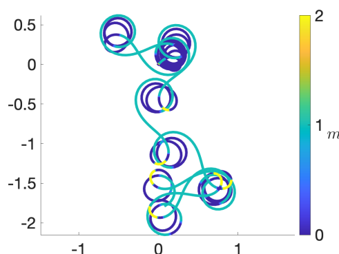
Figure 19. Center of mass trajectory for a wanderer with \alpha = -2.9 , \zeta = 0.12 , \beta = 0.2 , d_R = 0.05 , d_T = 0.05 , and Ca = 1.0 . Numerical simulations reveal behavior that is similar to run-and-tumble dynamics.
