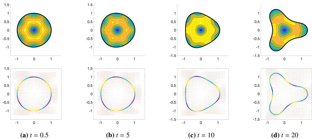
Figure 21. Dynamics of the m = 3 mode in a drop filled with a contractile active fluid with \alpha = 4.8 , \zeta = 0.5 , d_T = 0.01 , d_R = 0.005 , and Ca = 1 . Top row shows contours of the scalar nematic order parameter, plotted over the direction of the dominant eigenvectors; bottom row shows corresponding flow field, with the drop boundary color-coded by the interior limit of the vorticity at the interface. The columns progress in time from left to right, with the time indicated in the subcaption.
