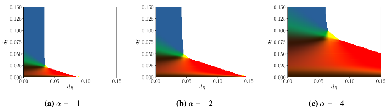
Figure 8. Mixture of unstable modes in the (d_R, d_T) plane at three different values of the activity parameter: \alpha = -1 for panel (a), \alpha = -2 for panel (b), and \alpha = -4 for panel (c), with \beta = 0.2 , \zeta = 0.1 , and Ca = 1 in all panels. See Figure 6 to interpret the color scale. Note the increased limits for both the x and y axes in panel (c).
